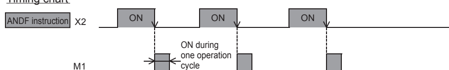
Timing chart
